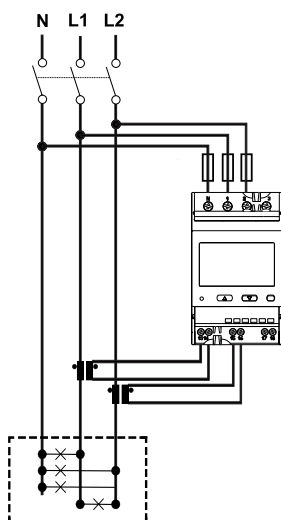
Fig. 11 Two-phase system with neutral (3-wire)
